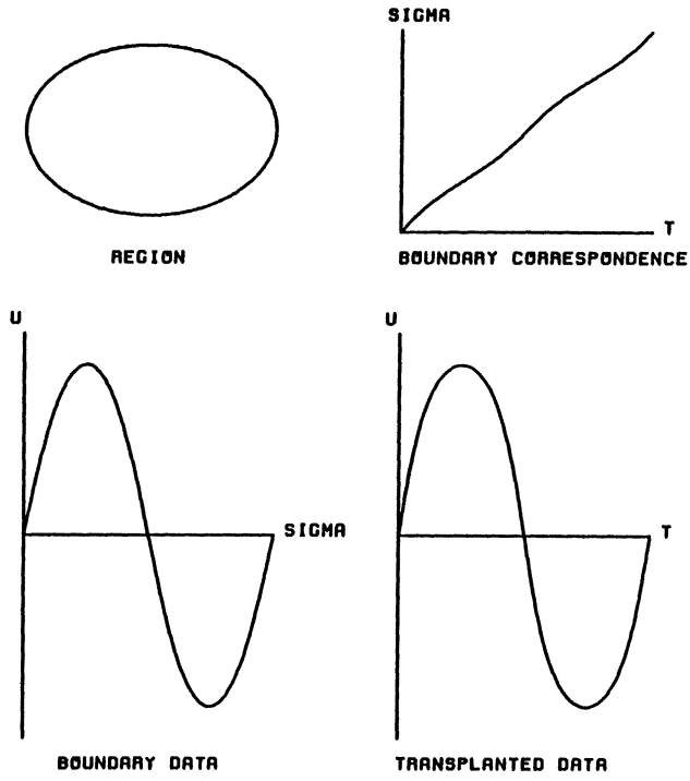
FIG. 13a. The effect of crowding on transplanted boundary data, \beta = .5 .
