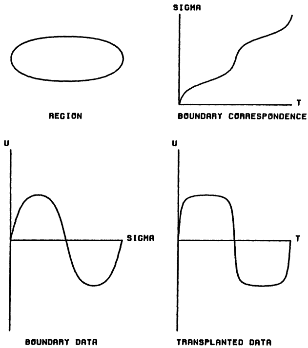
FIG. 13b. The effect of crowding on transplanted boundary data, \beta = .1 .
