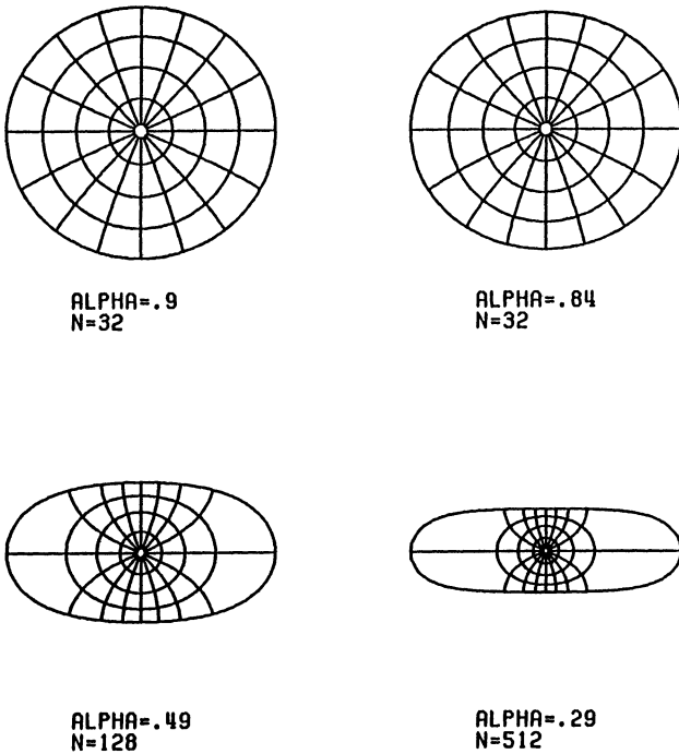
FIG. 7. Arctanh regions with Wegmann's method.
