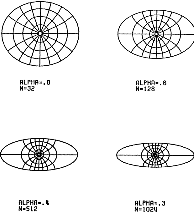
FIG. 9. Ellipses with Wegmann's method.
