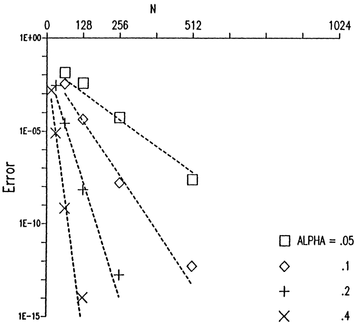
FIG. 2. Discretization errors for Wegmann's method for circles.
