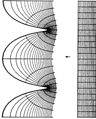
FIG. 11. Crowding for map of half plane, \text{Re } z \geq .2 by f(z) = 2 \log \sinh z/2 .
