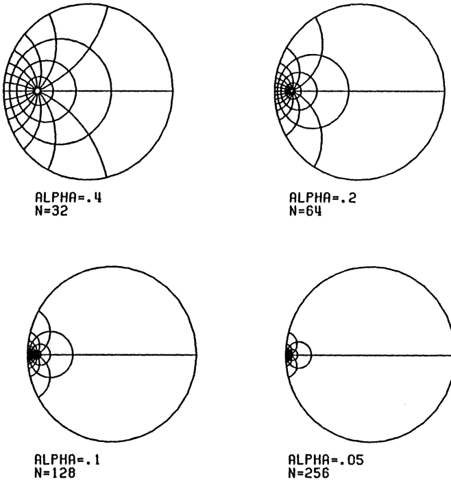
FIG. 1. Circles with Wegmann's method.
