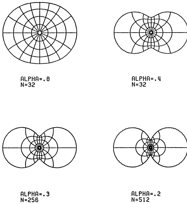
FIG. 3. Inverted ellipses with Wegmann's method.
